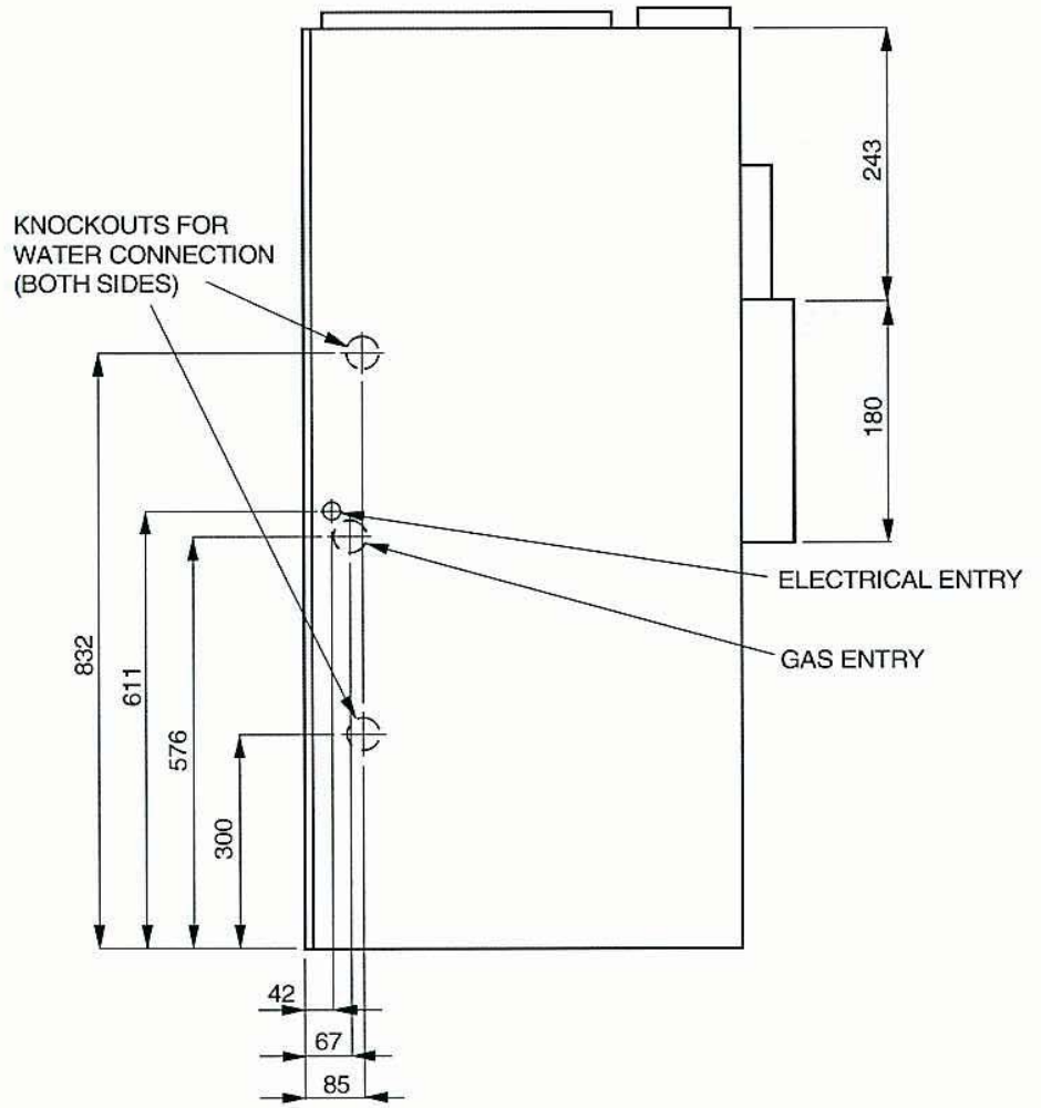
SIDE VIEW
