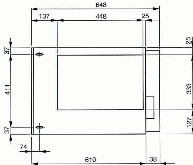
BASE VIEW
