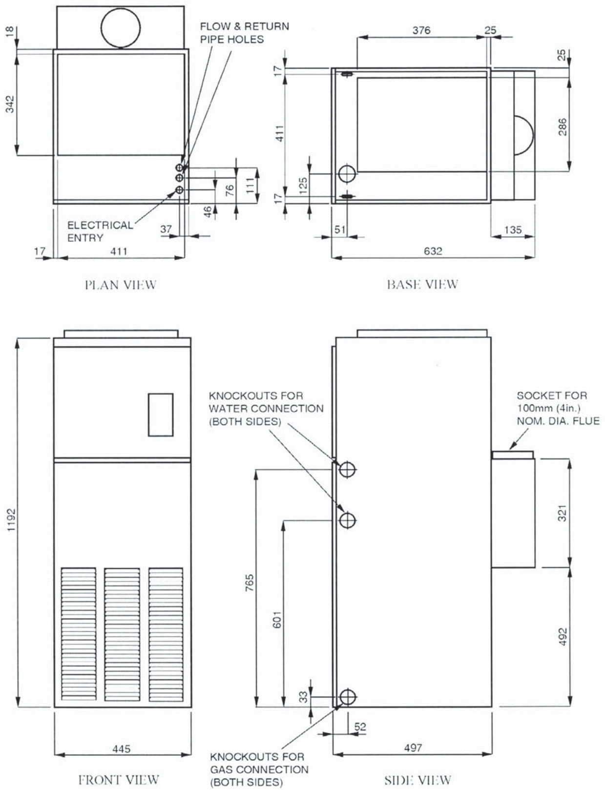
Fig. 8 Principal Dimensions
