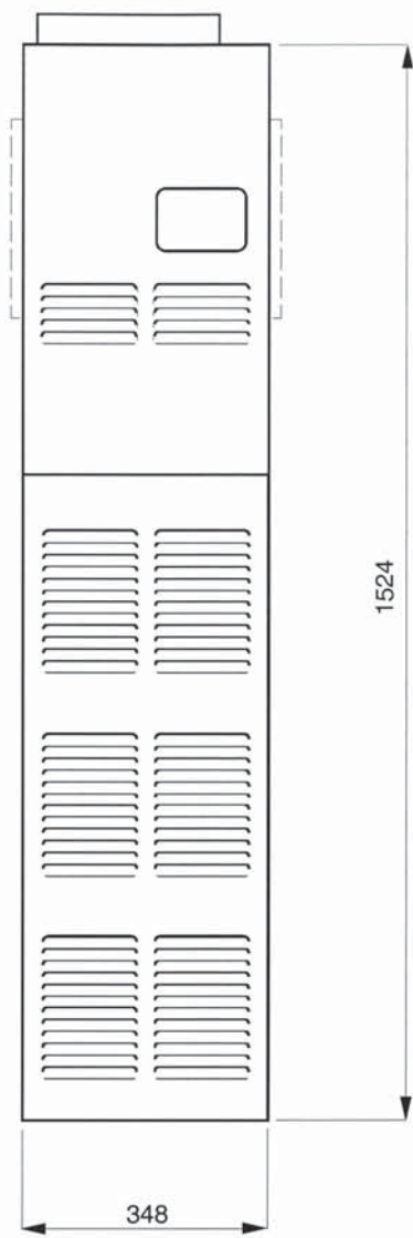
FRONT VIEW
