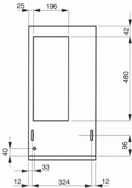
BASE VIEW
