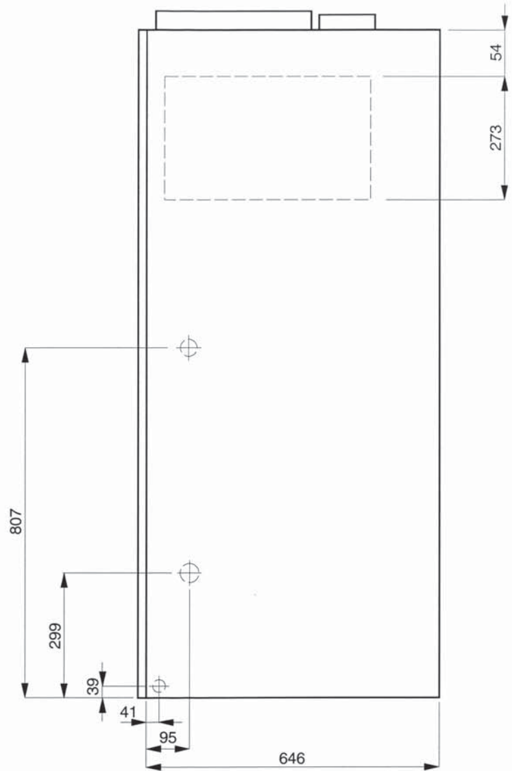
SIDE VIEW
