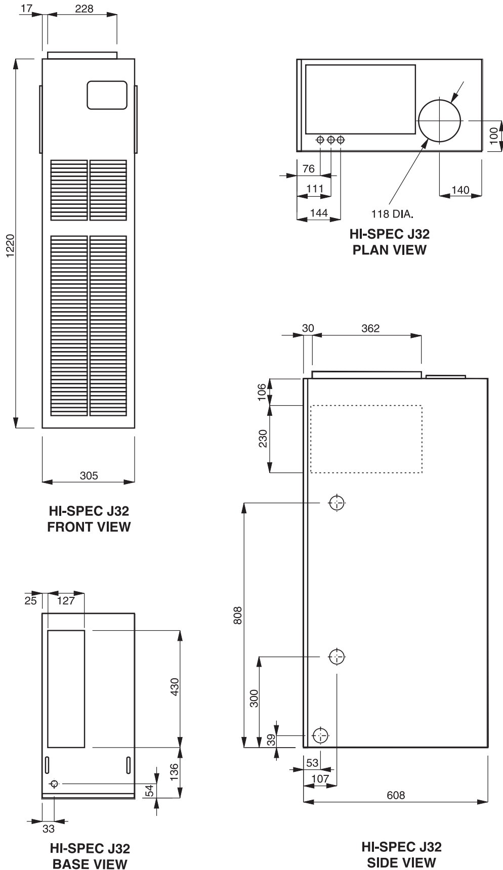
FIGURE 9 HI-SPEC J232 DIMENSIONS
