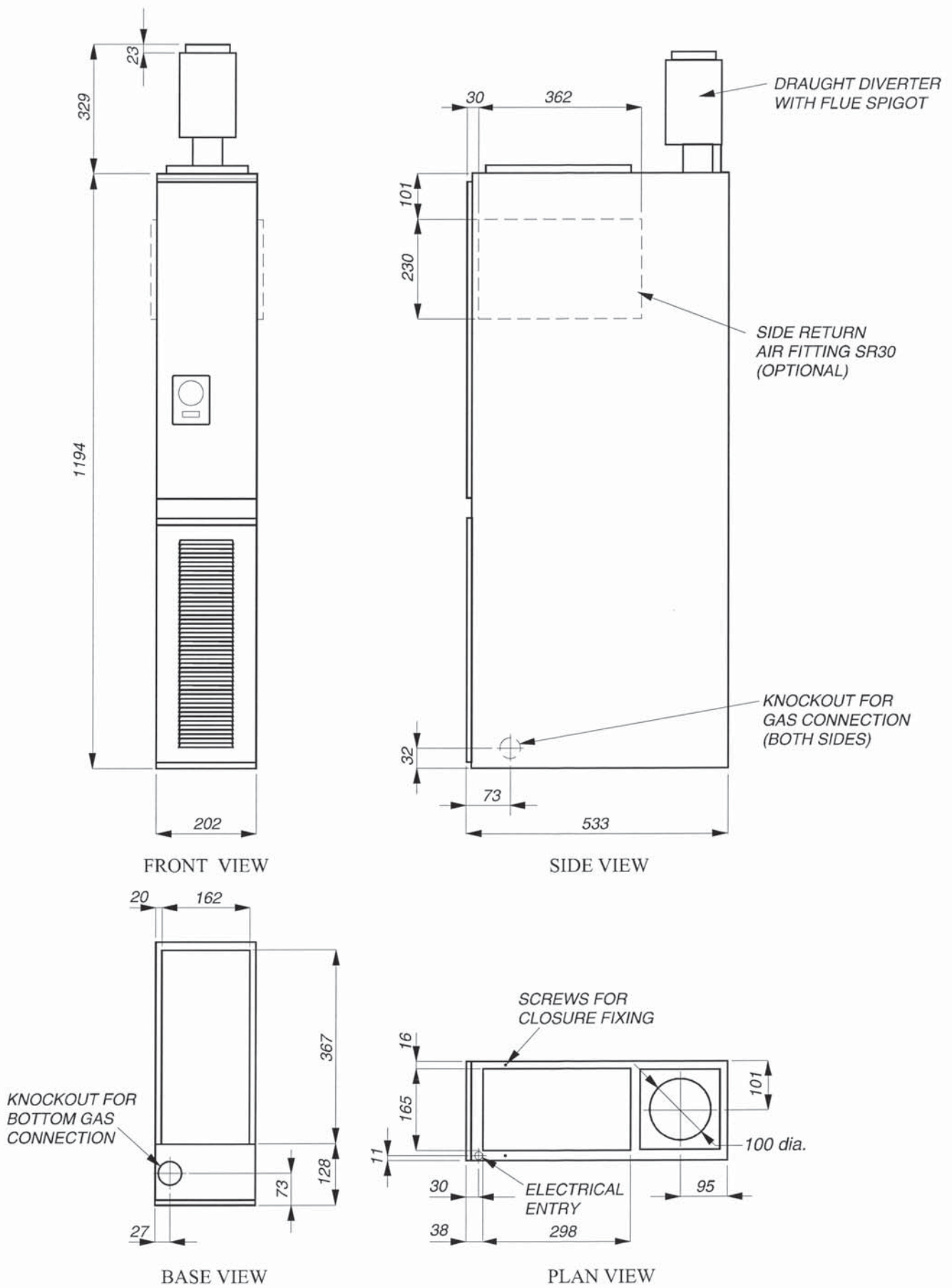
Fig. 7, PRINCIPAL DIMENSIONS (mm)
