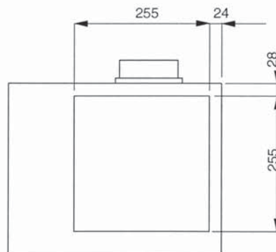
SPIGOT POSITION FROM FRONT
