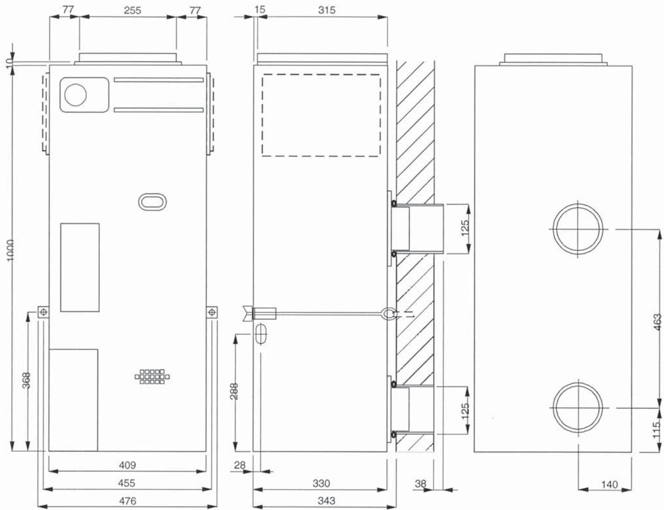
FRONT VIEW
